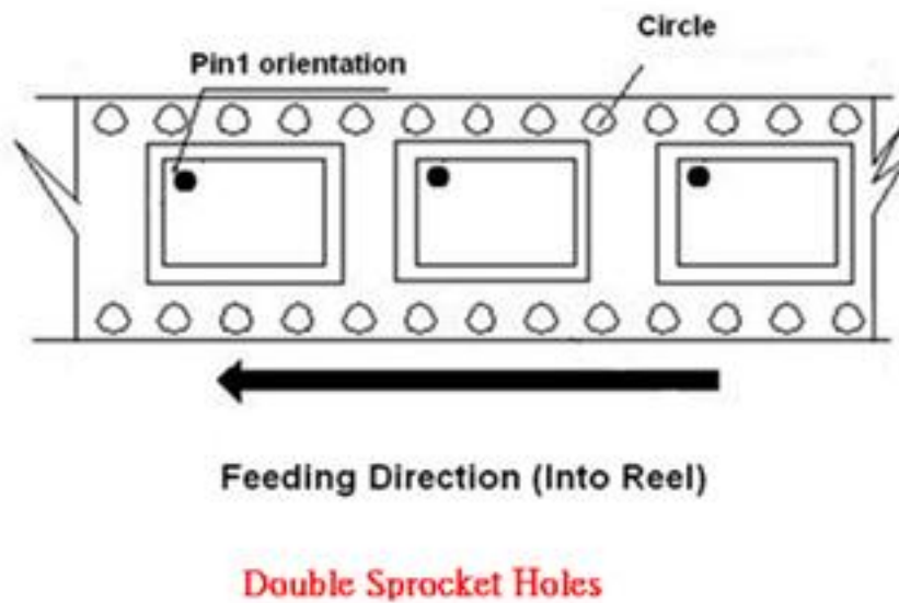
Figure 12 SN8000 Pin1 Orientation
