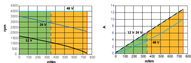
Speed / Torque 80180 SMi21 - Current / Torque 80180 SMi21
