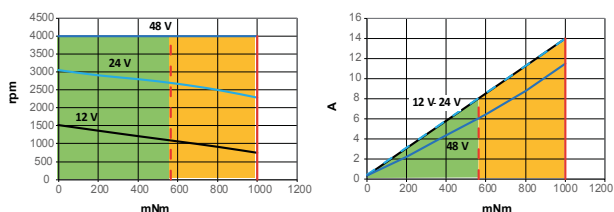
Speed / Torque 80280 SMi21- Current / Torque 80280 SMi21
