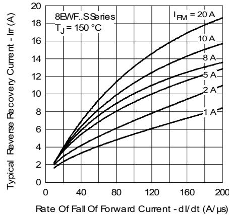
Fig. 13 - Recovery Current Characteristics, T_J = 150\text{ °C}
