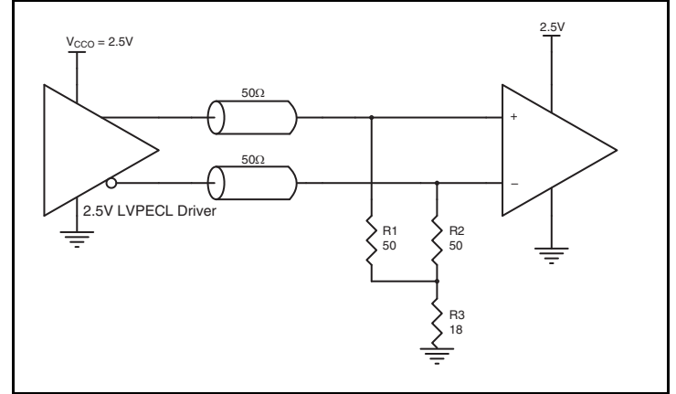
Figure 11C. 2.5V LVPECL Driver Termination Example
