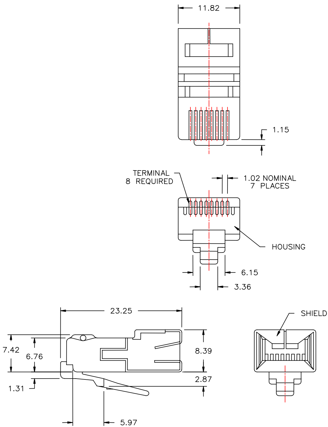
Figure 3 - 8 Position keyed Plug Mechanical Specification
