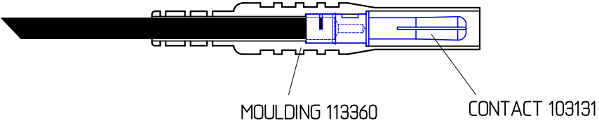
125070 OEM PLUG
