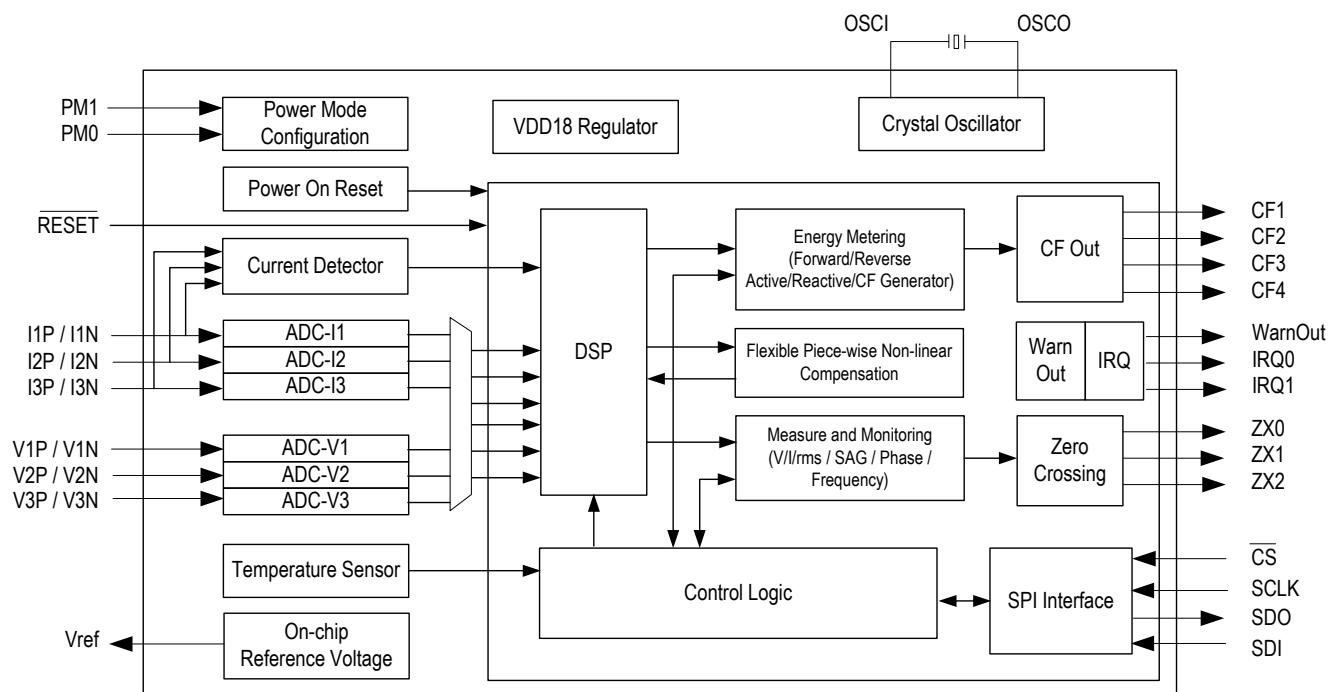
Figure-1 90E32AS Block Diagram
