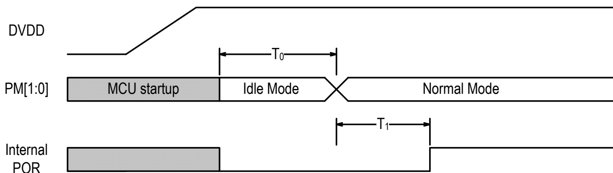
Figure-23 Power On Reset Timing (90E32AS and MCU are Powered on Simultaneously)
