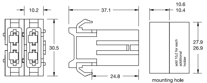
Dimensions in mm / Maße in mm
