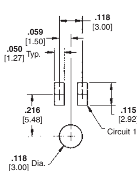
Recommended PC Board Layout * 2 Position
