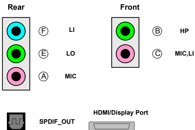
Figure 21. Port Configurations
