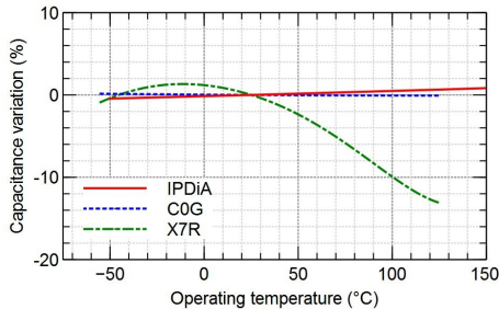
Fig.1: Capacitance variation vs temperature (for WBSC and MLCC technologies)
