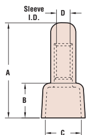
Part No. 2988** Features Extra Clearance Beyond Sleeve.
