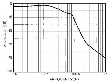
FMC-461 Typical Amplitude Response vs. Frequency
