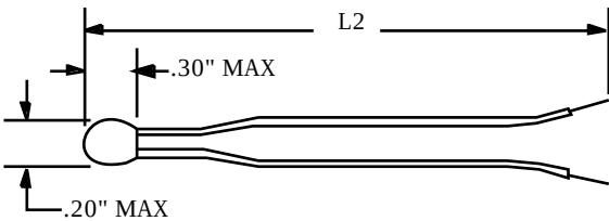
Epoxy-Encapsulated Thermistor
