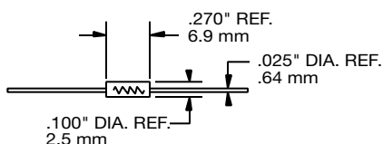
YSI 44300 Series Resistor
