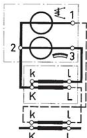
With separate current transformer
