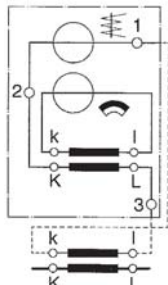
With built in current transformer
