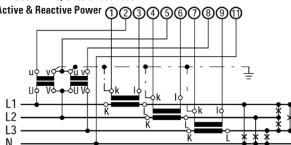
3-Phase 4-Wire, Unbalanced Load Active & Reactive Power
