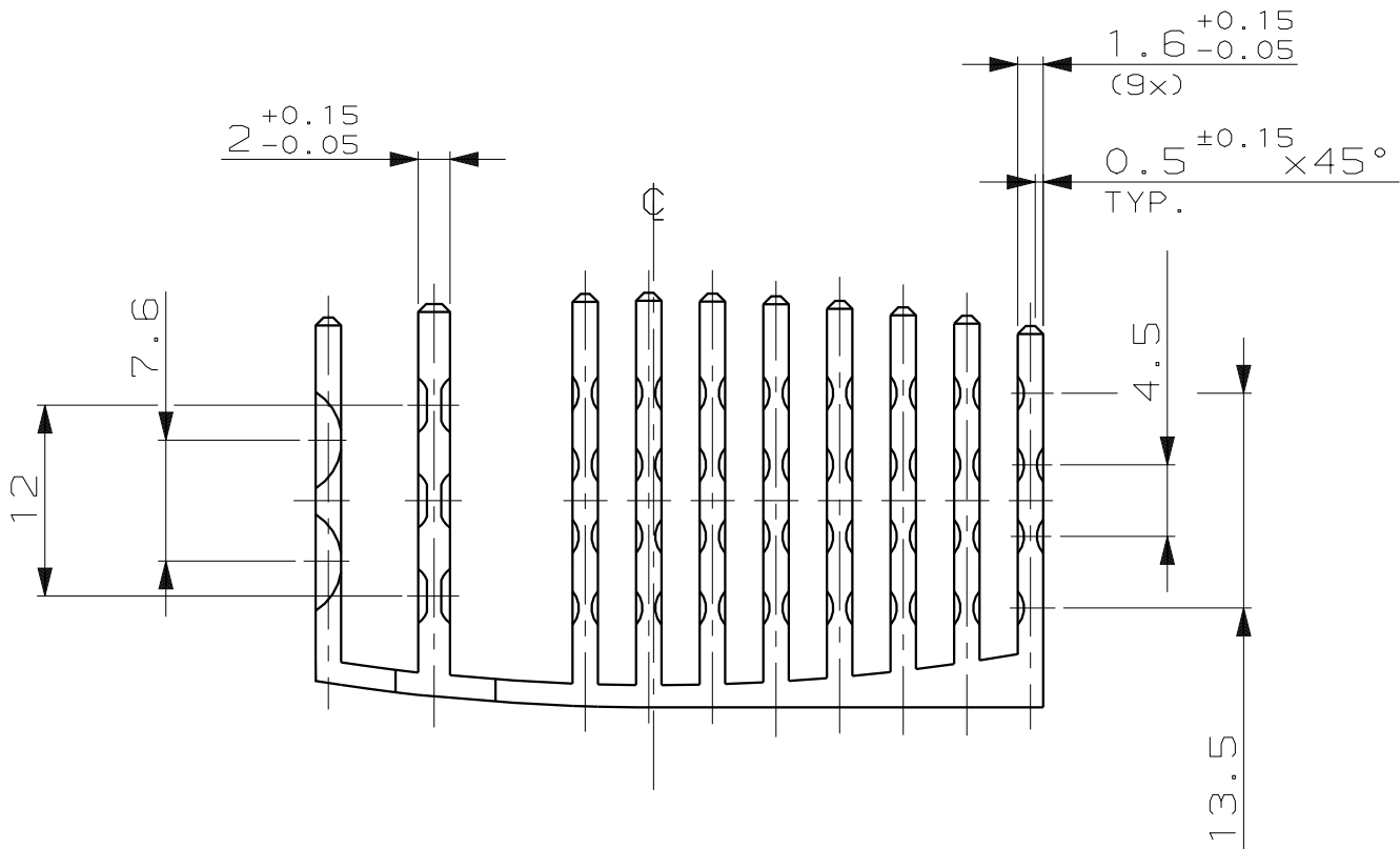
Ansicht "Z" VIEW "Z"
