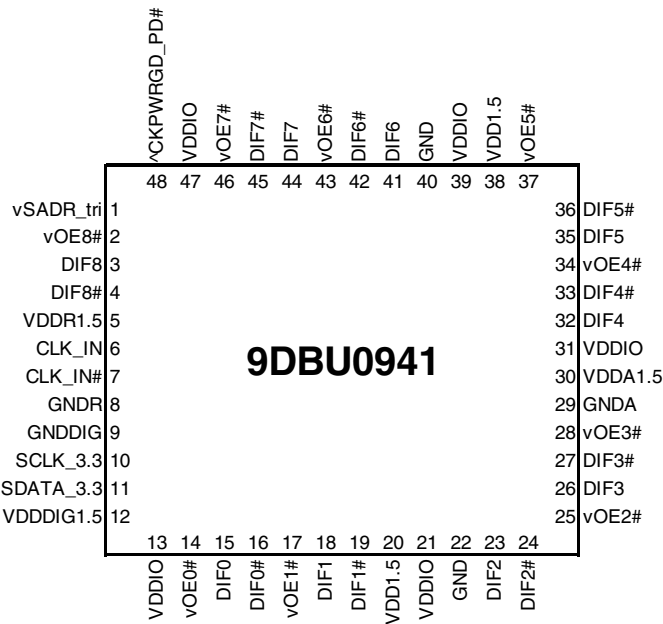
48-pin VFQFPN, 6x6 mm, 0.4mm pitch
