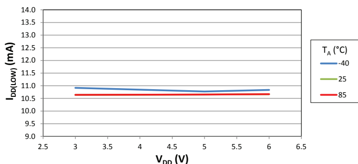
Average Low Supply Current versus Supply Voltage
