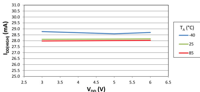
Average High Supply Current versus Supply Voltage
