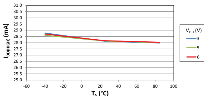
Average High Supply Current versus Ambient Temperature
