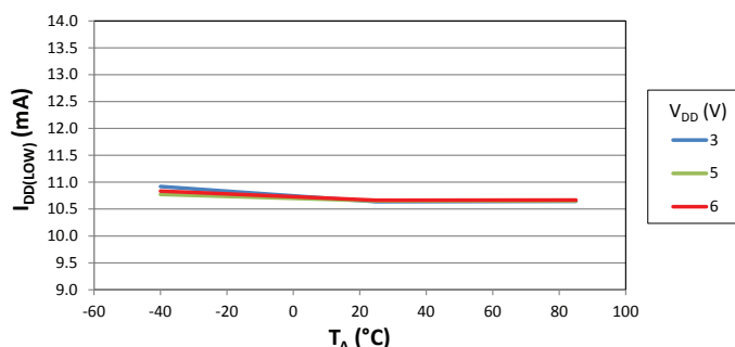
Average Low Supply Current versus Ambient Temperature
