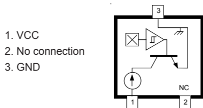
Package LH, 3-pin SOT
