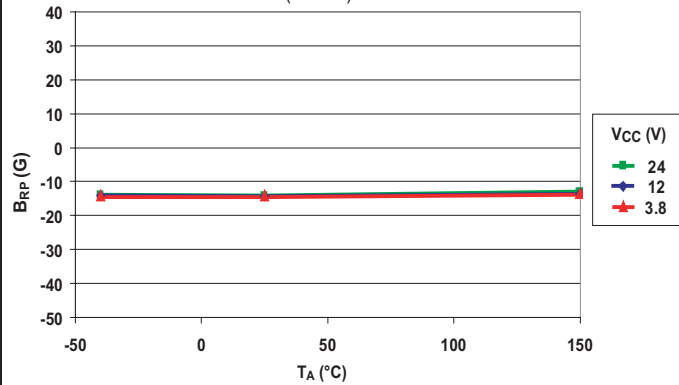
Release Point versus Ambient Temperature (A1201)
