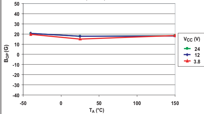
Operate Point versus Ambient Temperature (A1201)
