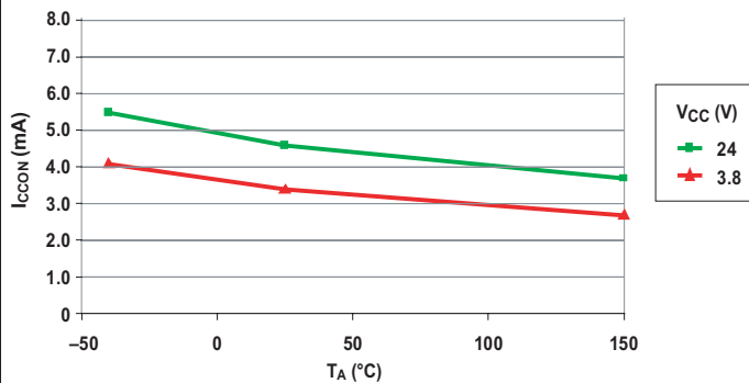
Supply Current (On) versus Ambient Temperature (A1201/02/03/04)
