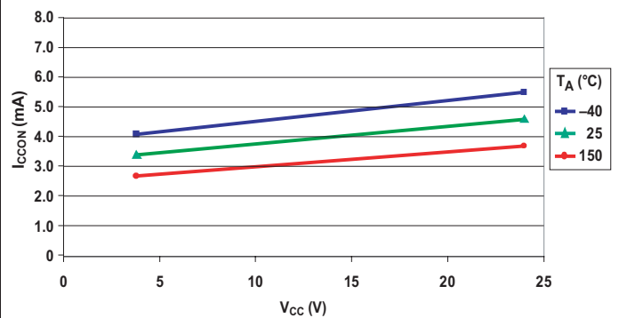
Supply Current (On) versus Supply Voltage (A1201/02/03/04)
