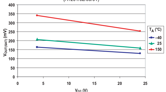
Output Voltage (On) versus Supply Voltage (A1201/02/03/04)
