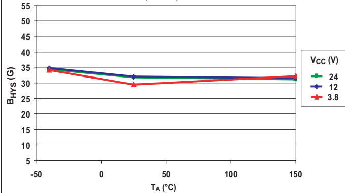
Hysteresis versus Ambient Temperature (A1201)
