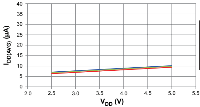
Average Supply Current vs. Supply Voltage
