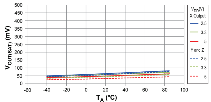
Average Low Output Voltage vs. Ambient Temperature
