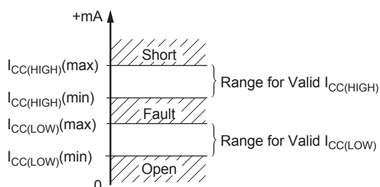
Figure 2: Diagnostic Characteristics of Supply Current Values.
