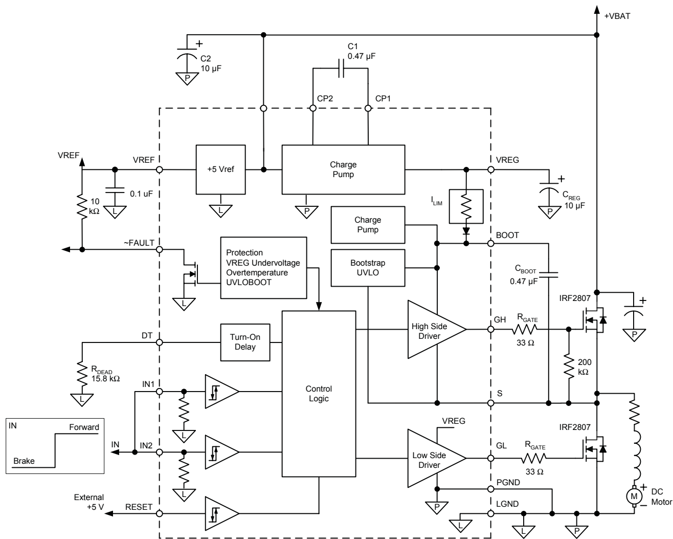
Diagram A. Dependent drivers. Unidirectional motor control with braking and dead time. T_{DEAD} = 1 \mu s ; Q_{TOTAL} = 160 nC .
