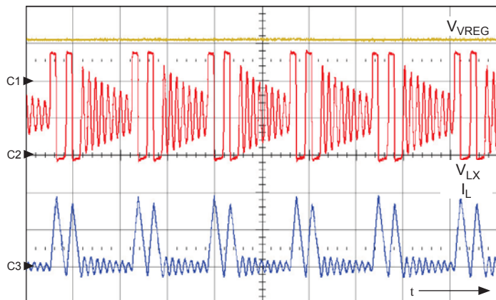
PWM at V_{BAT} = 12 V with a VREG 25 mA load; shows V_{VREG} (ch1, 5 V/div.), V_{LX} (ch2, 5 V/div.), I_L (ch3, 100 mA/div.), t = 2 μs/div.
