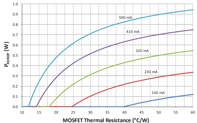
Figure 10. R_{DROD} Dissipation versus MOSFET thermal resistance at various V33 regulator maximum current settings, I_{V33ILIM}
