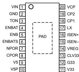
Pin-out Diagram
