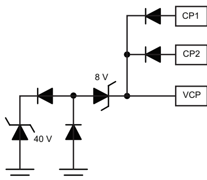
Figure 20: VCP, CP1, CP2
