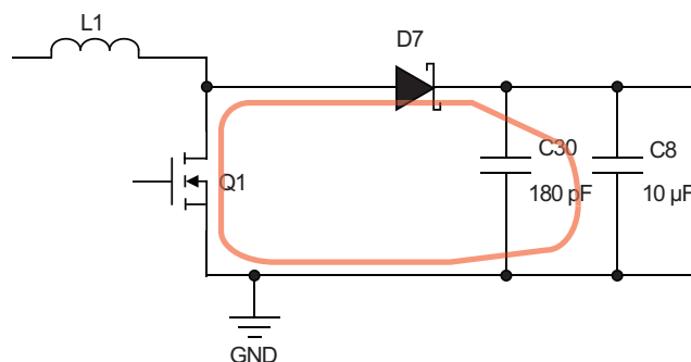
Figure 14: Boost Output Loop
