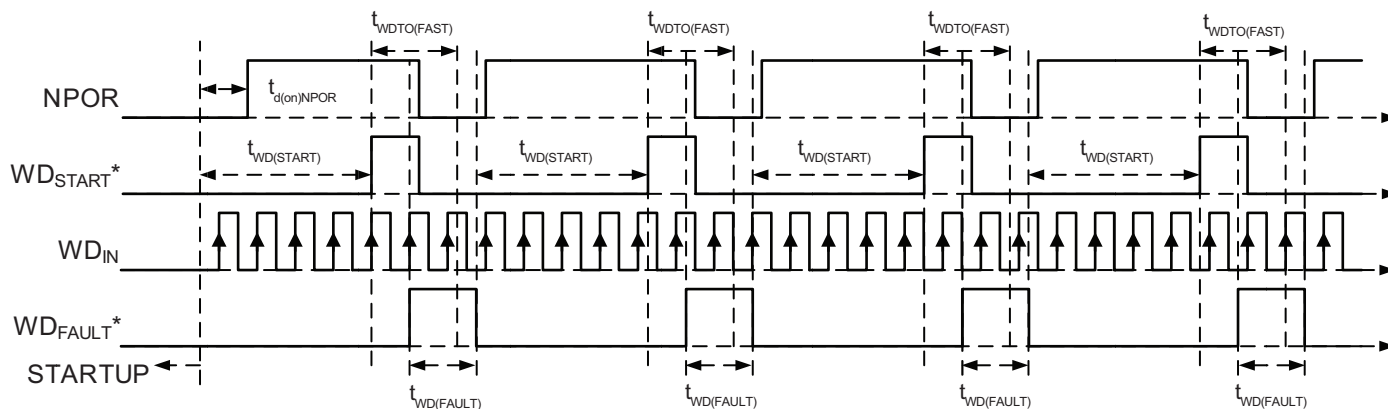
Figure 10: Window Watchdog Timer operation during fast clock fault * signal is internal to A4409
