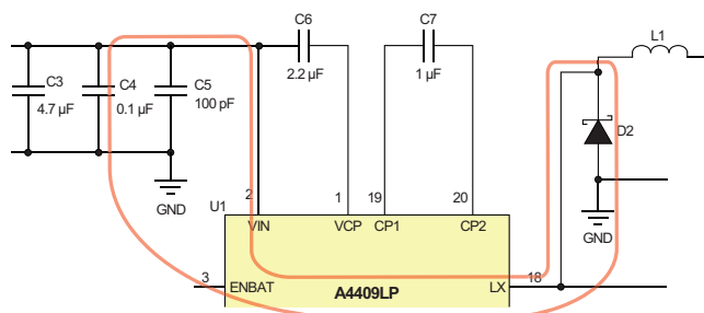
Figure 12: Buck High di/dt Loop
