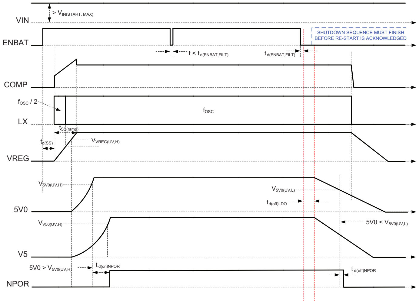
Figure 1: Startup and Shutdown Sequence
