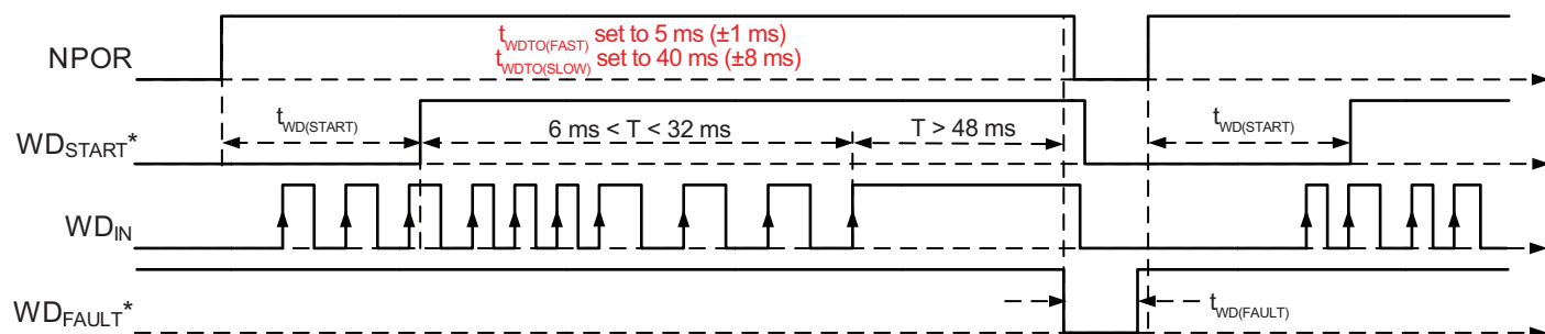
Figure 8: Window Watchdog Timer SLOW Fault, T = \text{WD}_{IN} period
