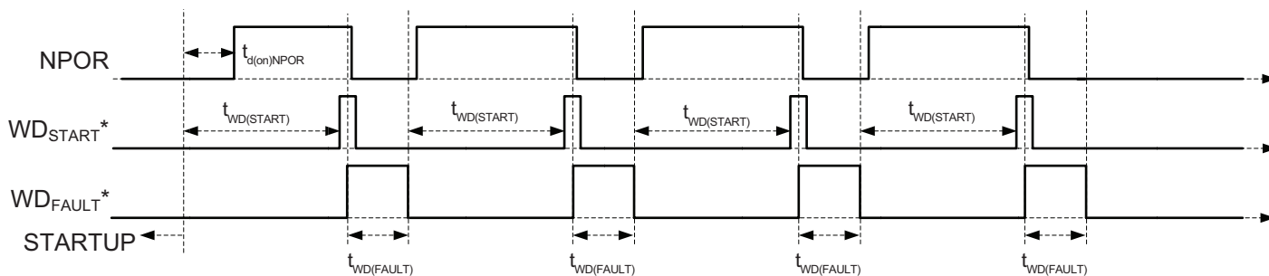
Figure 11: Window Watchdog Timer operation during R_{ADJ} fault * signal is internal to A4409
