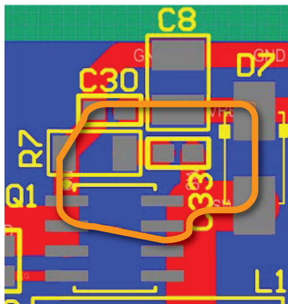
Figure 15: Boost High di/dt Loop
