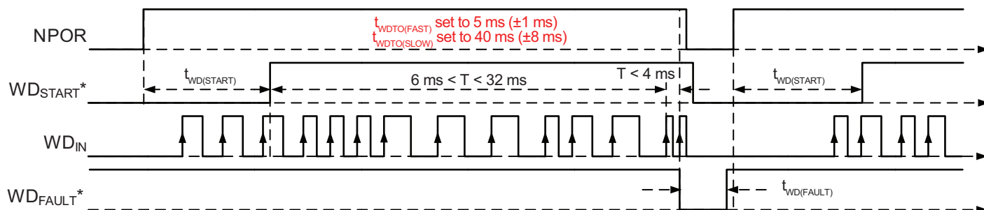
Figure 7: Window Watchdog Timer FAST Fault, T = \text{WD}_{IN} period
