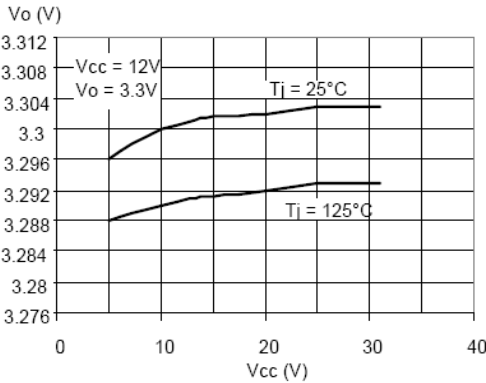
Figure 23. Line regulation
