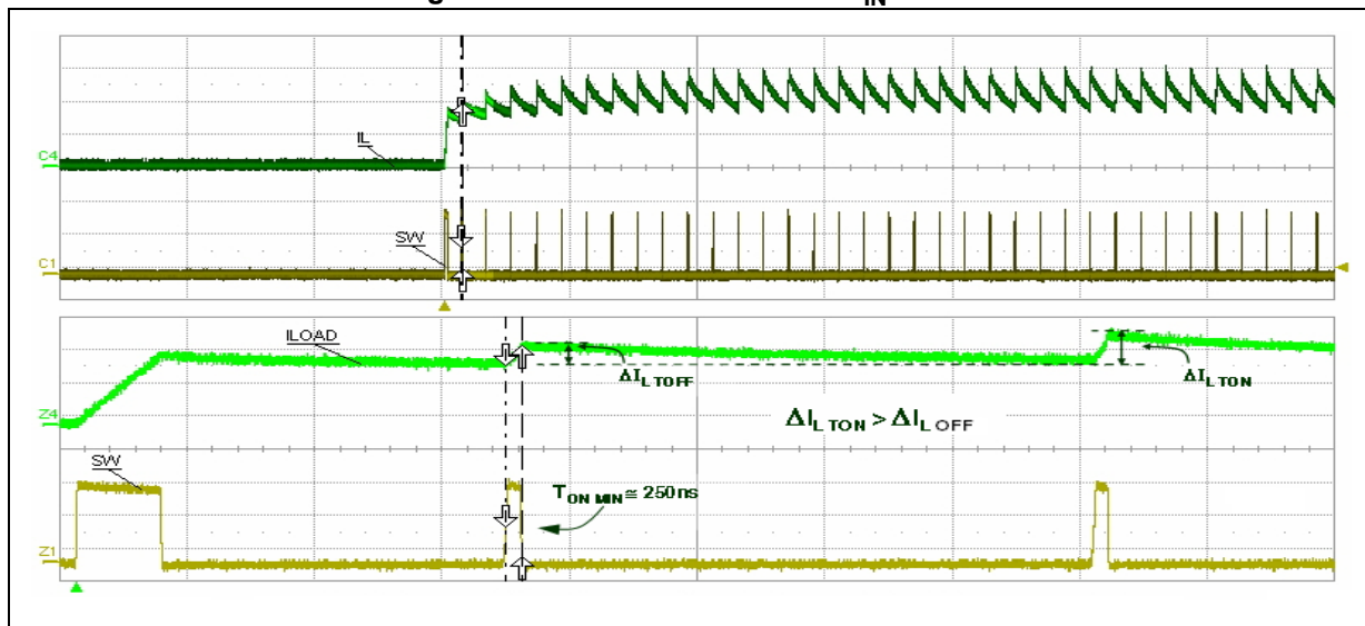
Figure 15. Short-circuit current V_{IN} = 36\text{ V}
