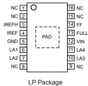
Pin-out Diagrams
