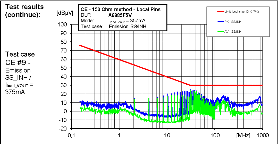
Figure 73. CE 150R at SS/INH test point (see Figure 66 on page 74 ) at 75% I LOAD
