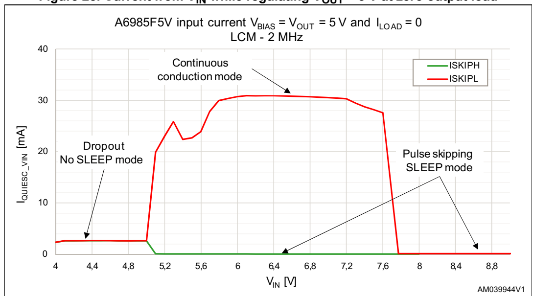
Figure 28. Current from V_{IN} while regulating V_{OUT} = 5 V at zero output load
