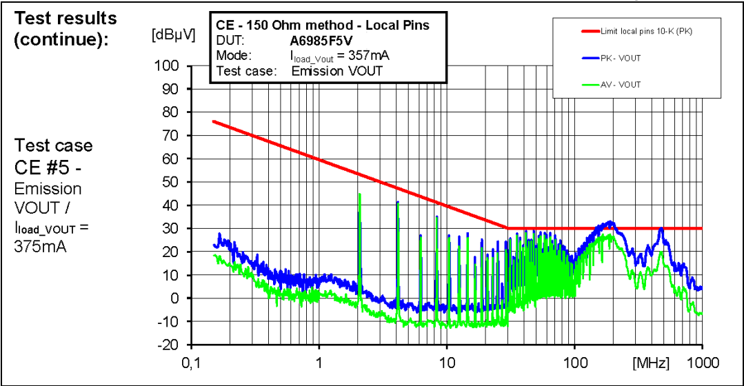
Figure 69. CE 150R at VOUT test point (see Figure 66) at 75% I LOAD
