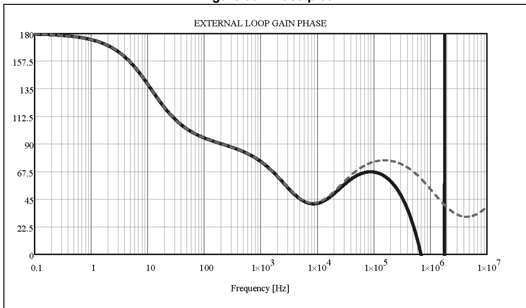
Figure 39. Phase plot
