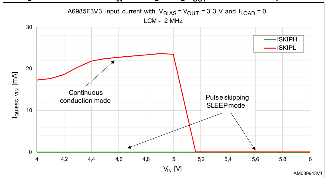
Figure 27. Current from V_{IN} while regulating V_{OUT} = 3.3 V at zero output load
