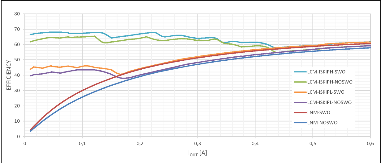
Figure 60. A6985F3V3 efficiency curves: V_{IN} = 24V - f_{sw} = 2\text{ MHz}
