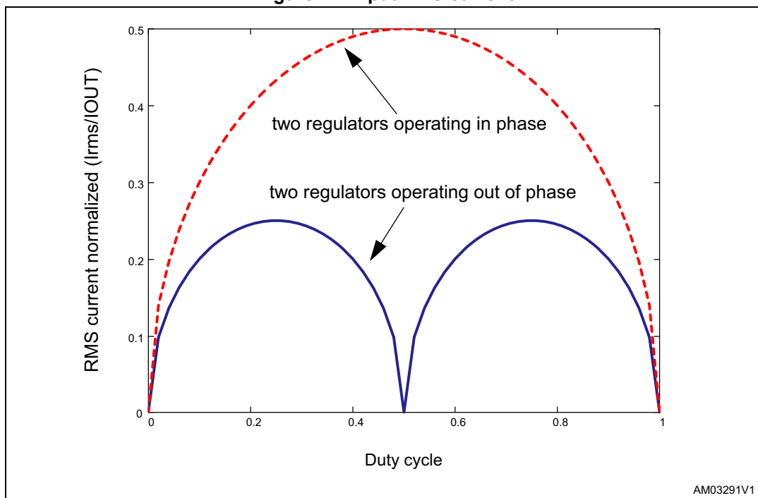
Figure 42. Input RMS current
