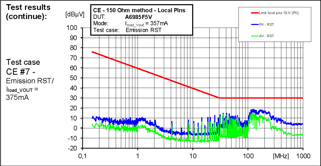
Figure 71. CE 150R at RST test point (see Figure 66) at 75% I LOAD
