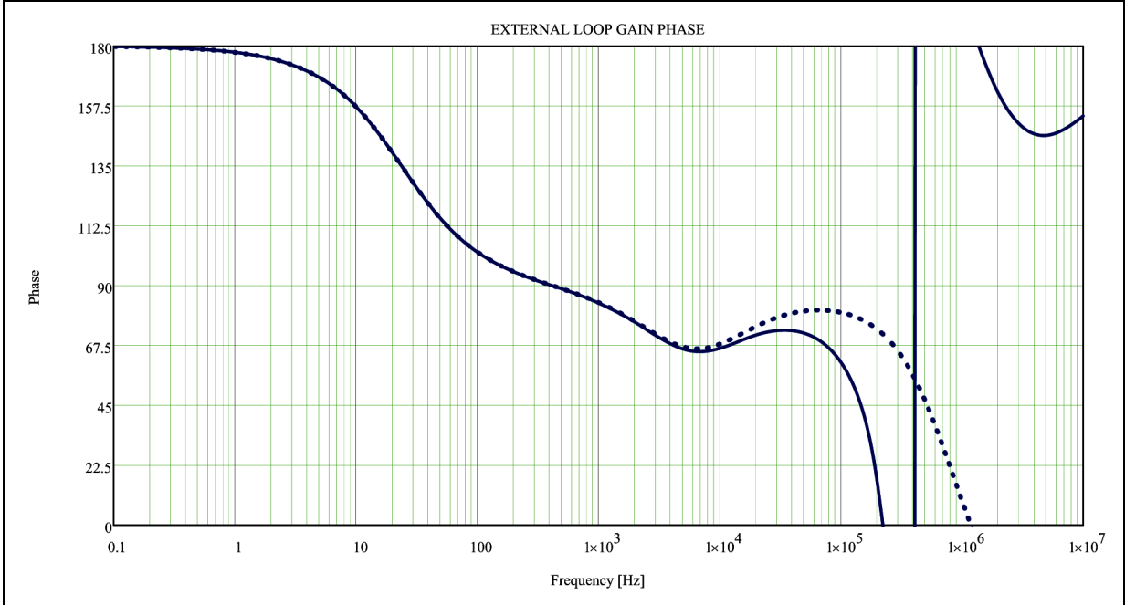
Figure 33. Phase plot
