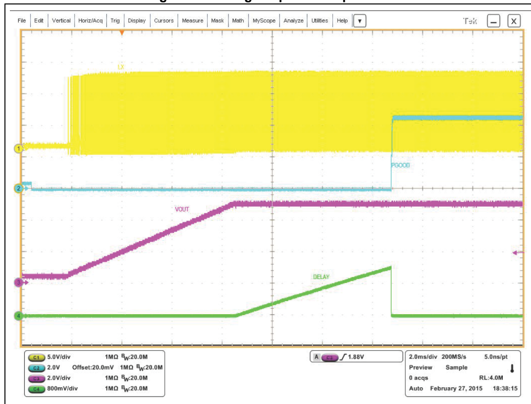
Figure 37. Voltage supervisor operation
