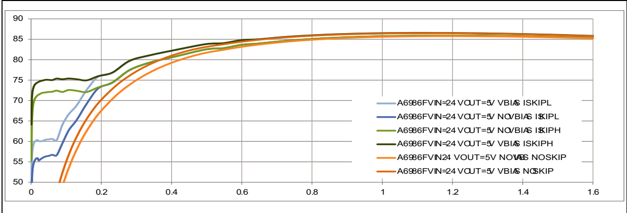
Figure 56. Efficiency curves: V_{IN} = 24\text{ V} - V_{OUT} = 5\text{ V} - f_{sw} = 500\text{ kHz}
