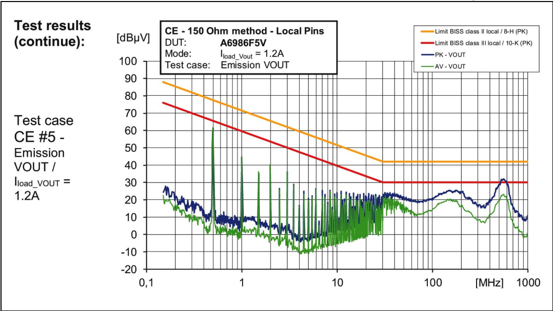
Figure 61. CE 150R at VOUT test point (see Figure 58 ) at 80% I LOAD
