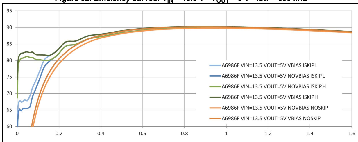
Figure 52. Efficiency curves: V_{IN} = 13.5\text{ V} - V_{OUT} = 5\text{ V} - f_{sw} = 500\text{ kHz}
