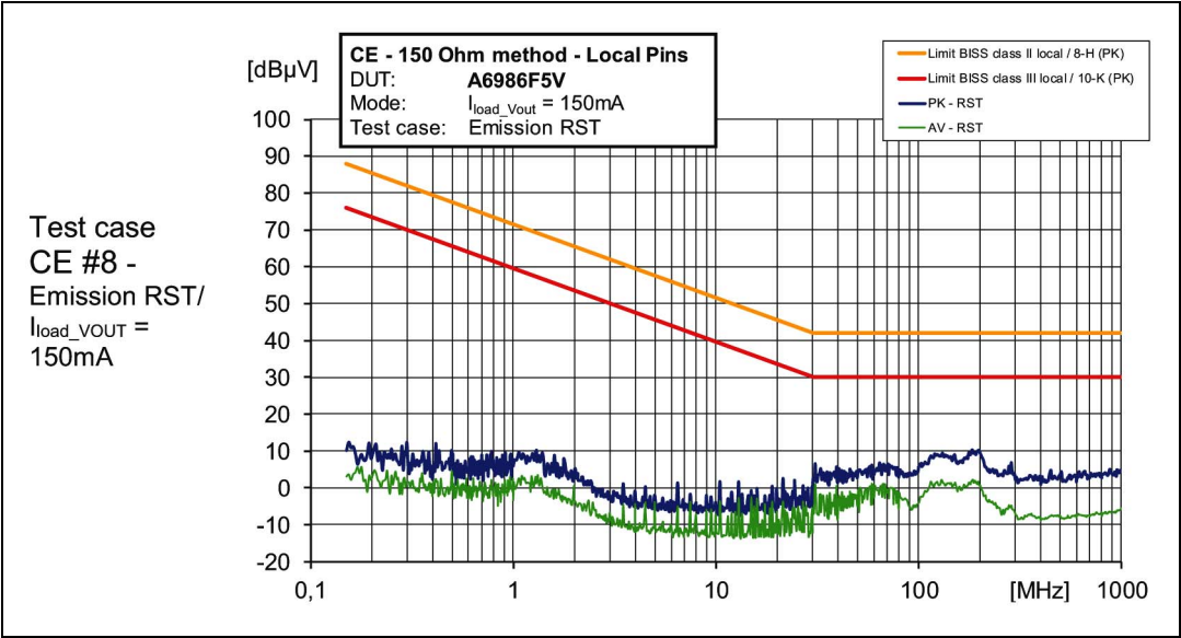
Figure 66. CE 150R at SS/INH test point (see Figure 58 ) at 10% I_{LOAD}
