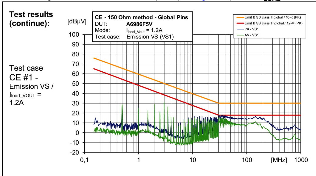
Figure 60. CE 150R at VS1 test point (see Figure 58 ) at 10% I_{LOAD}
