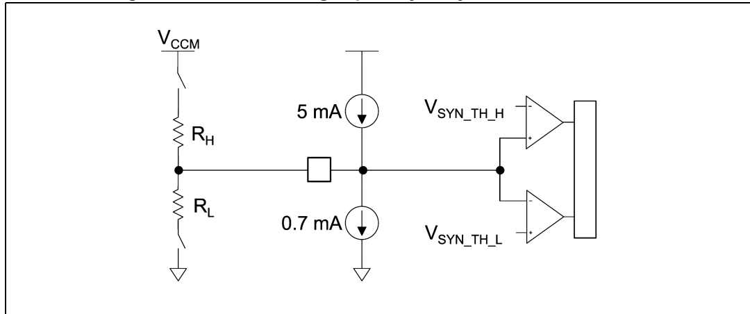
Figure 44. Master driving capability to synchronize the A6986
