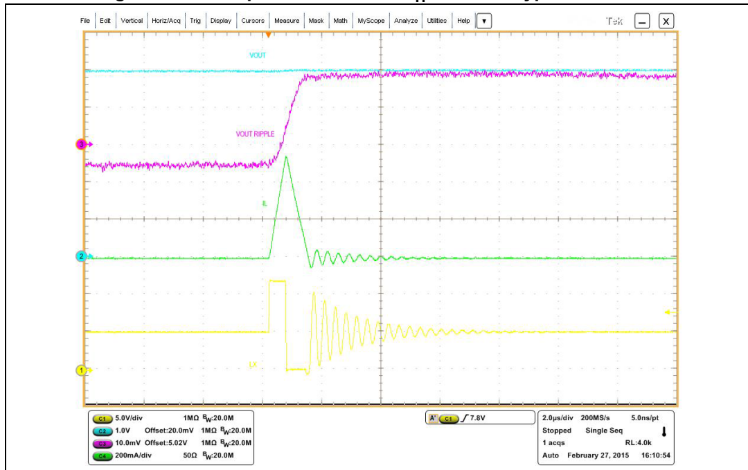
Figure 17. LCM operation with ISKIP_H = 200 \text{ mA typ.} at zero load
