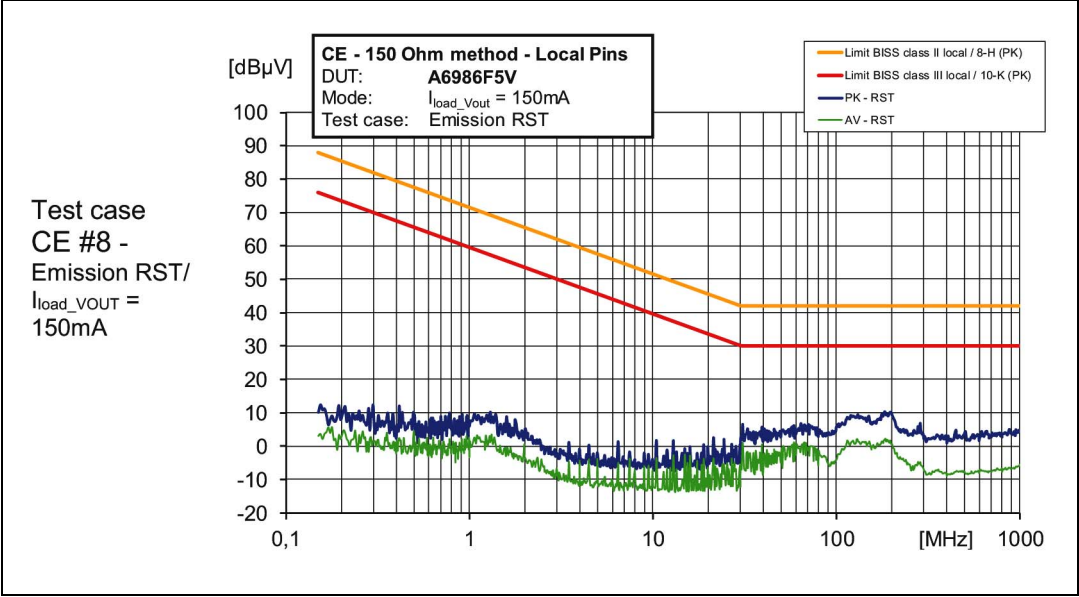
Figure 64. CE 150R at RST test point (see Figure 58 ) at 10% I LOAD
