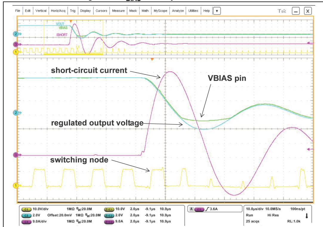
Figure 27. V_{BIAS} in heavy short-circuit event
