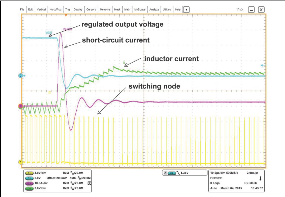
Figure 25. Output voltage oscillations during heavy short-circuit
