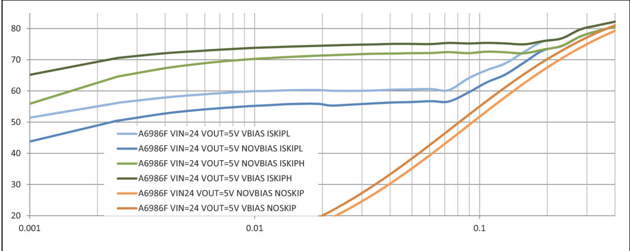
Figure 57. Efficiency curves: V_{IN} = 24\text{ V} - V_{OUT} = 5\text{ V} - f_{sw} = 500\text{ kHz} (log scale)
