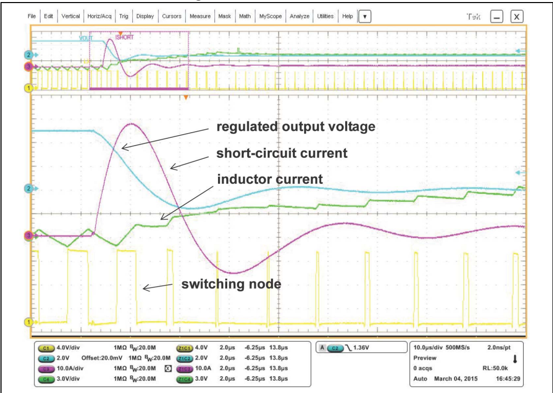
Figure 26. Zoomed waveform
