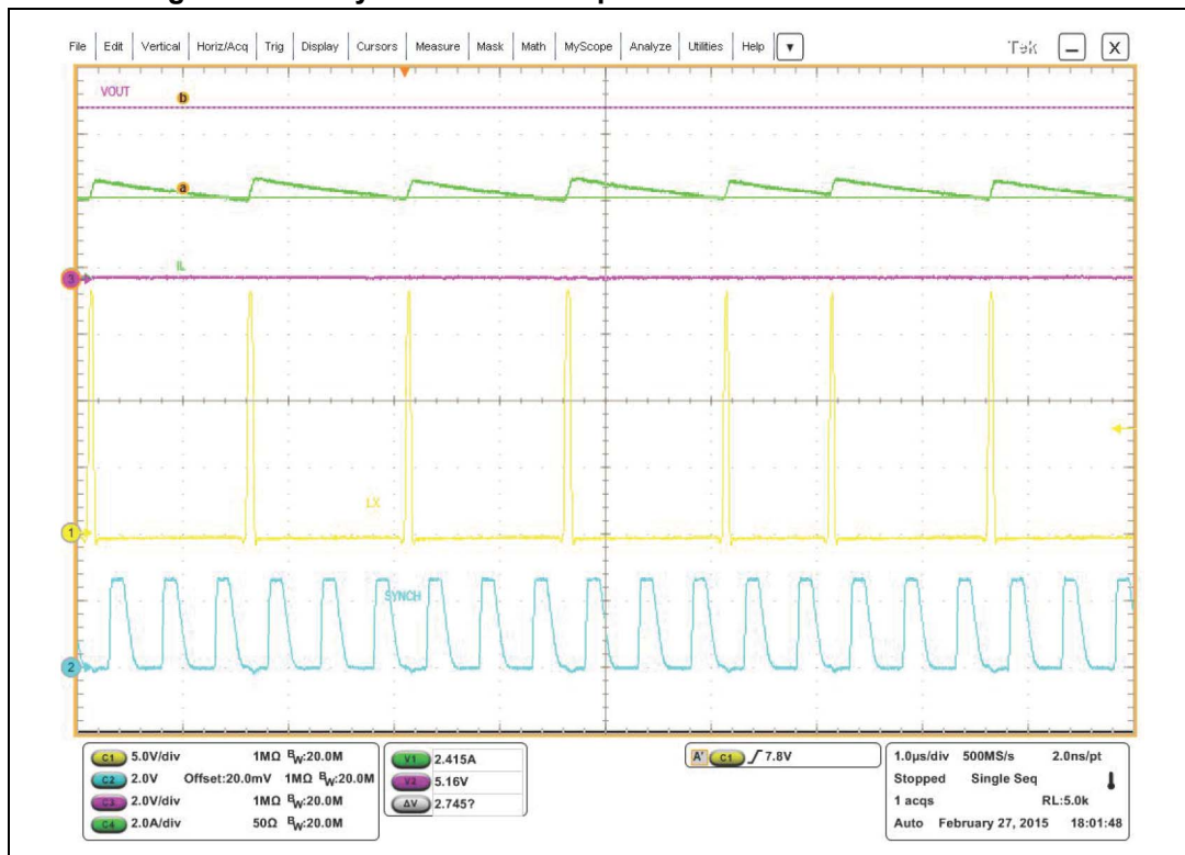
Figure 23. Valley current sense operation in overcurrent condition
