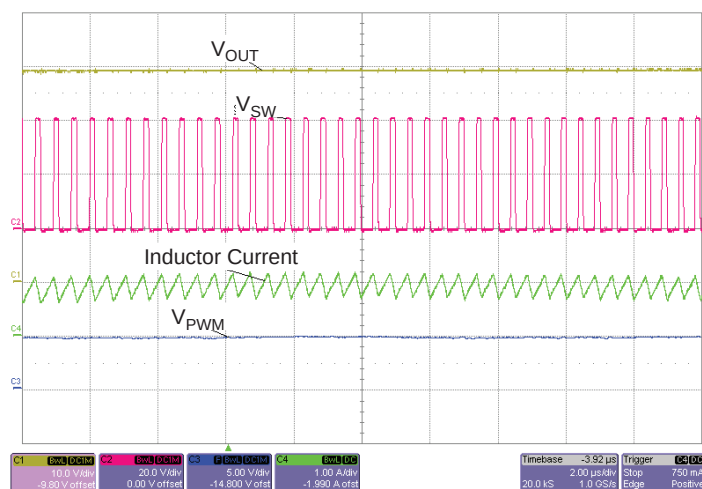
Figure 29: Normal Operation of Switch Node ( V_{SW} ), Inductor Current, and Output Voltage ( V_{OUT} )
