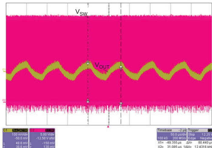
Figure 38: Output Voltage Ripple Frequency Due to Dithering = 12.4 kHz at V_{IN} = 12 V, and PWM Ratio = 100%
