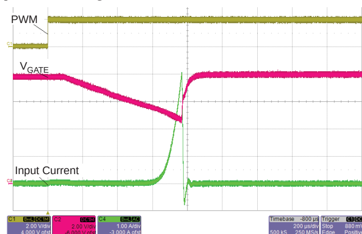
Figure 33: Startup into Output Shorted to GND fault. Input OCP tripped at 4 A ( R_{SC} = 0.024 \text{ W} , R_{adj} = 383 \text{ } \Omega )
