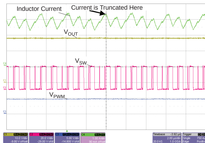
Figure 30: Cycle-by-Cycle Current Limit
