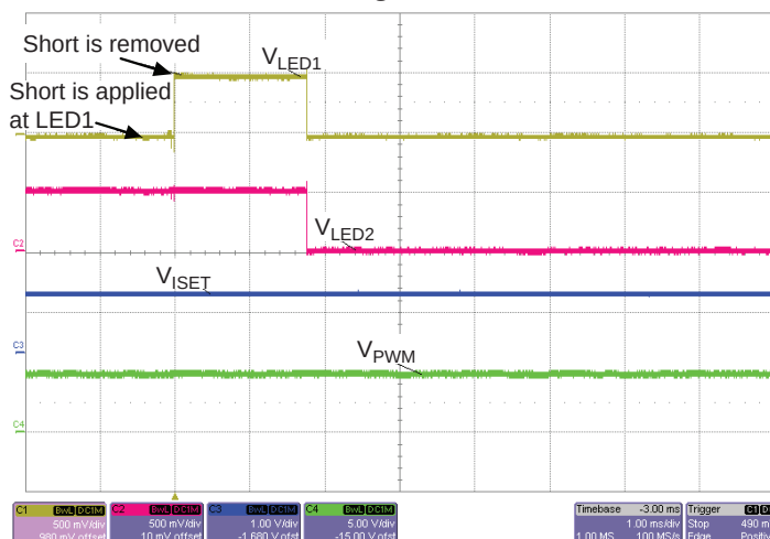
Figure 6: One LED Pin is Shorted to GND. The IC will not proceed with power up until LED pin is released, at which point the LED pin is checked to see if it is used.
