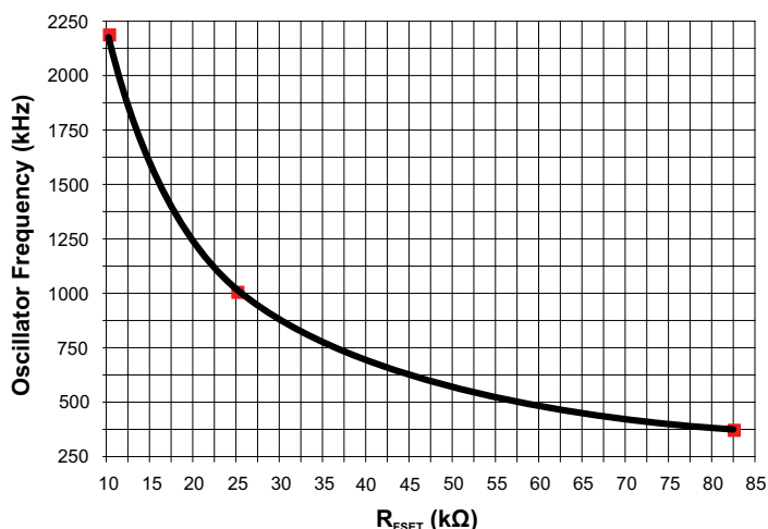
Figure 8. PWM Switching Frequency versus R_{FSET}
