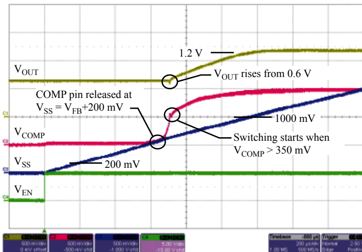
Figure 4: Startup to V_{OUTx} = 1.2 V, 2.0 A, with V_{OUT} pre-biased to 0.6 V
