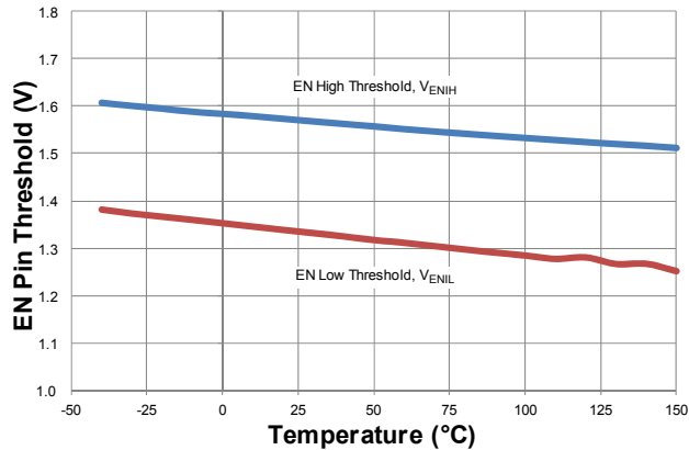
Enable High and Low Thresholds versus Temperature
