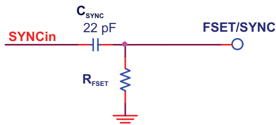
Figure 2: FSET/SYNC AC-Coupling
