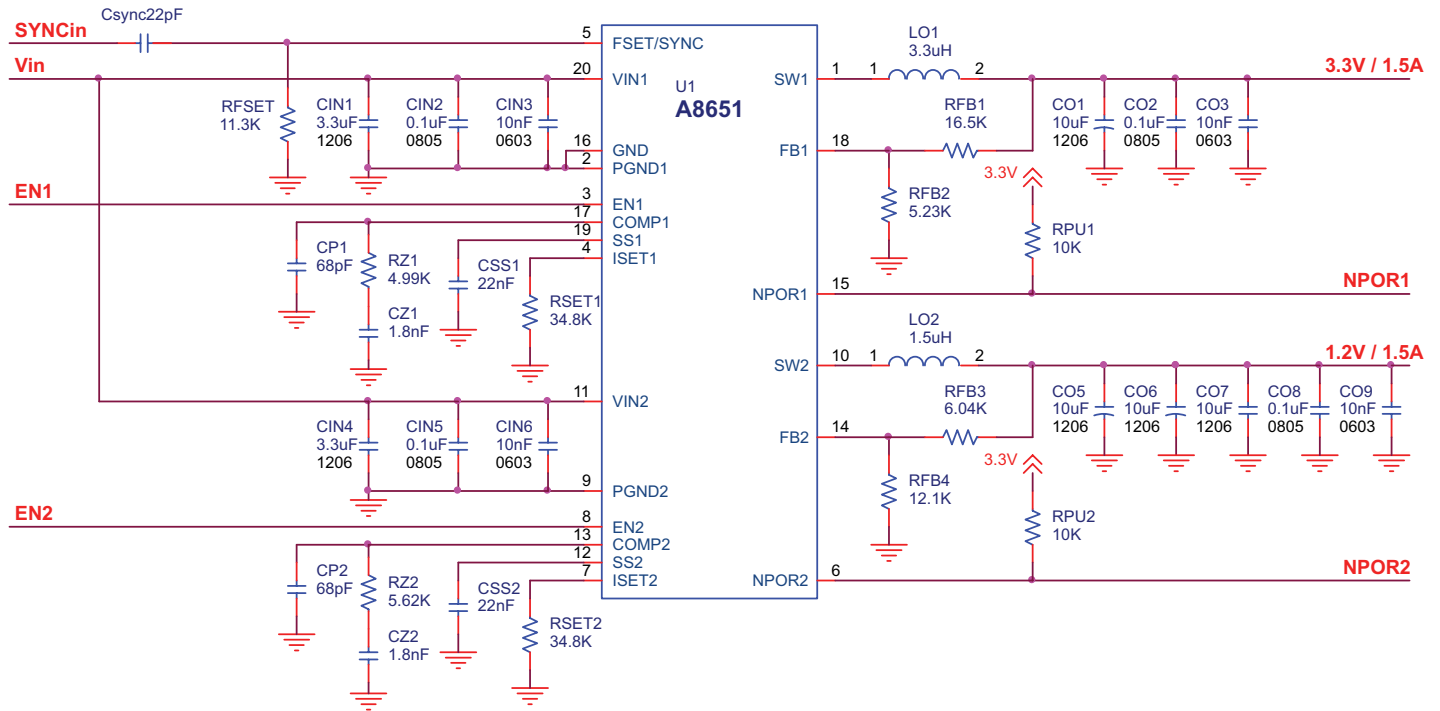
Figure 15: Typical Application Circuit for V_{IN} = 5\text{ V} at T_A = 125^\circ\text{C} : V_{OUT} = 3.3\text{ V}/1.5\text{ A} and 1.2\text{ V}/1.5\text{ A} at 2\text{ MHz} C_{SYNC} are only required if synchronizing to an external clock
