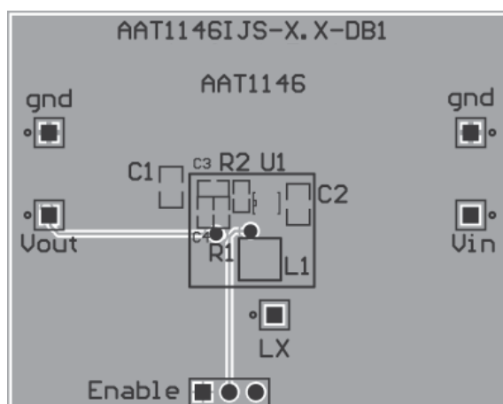
Figure 4: AAT1146 Evaluation Board Bottom Side Layout.
