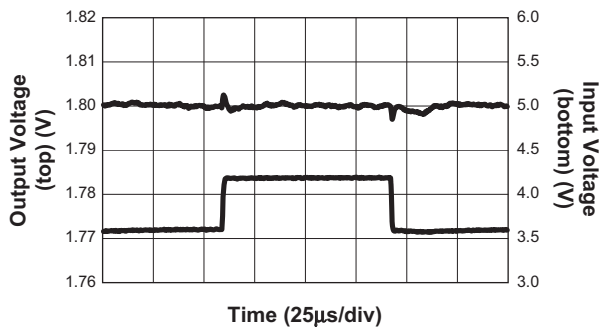
Line Response
