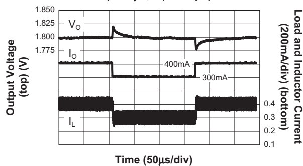
Load Transient Response (300mA to 400mA; V_{IN} = 3.6V ; V_{OUT} = 1.8V ; C_1 = 10\mu F ; C_4 = 100pF )
