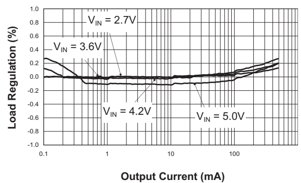
Load Regulation
