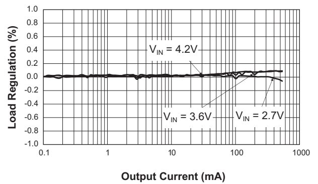
Load Regulation
