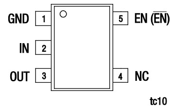
Figure 4. AAT3222 Pinout 5-Pin SOT23-5 (Top View)
