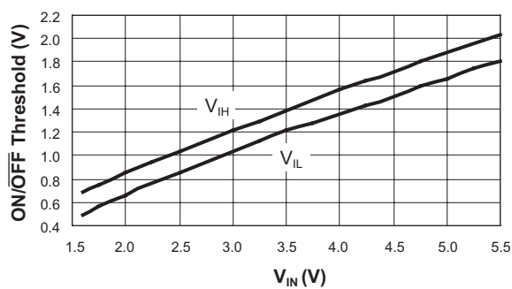
ON/OFF Threshold vs. V_{IN}
