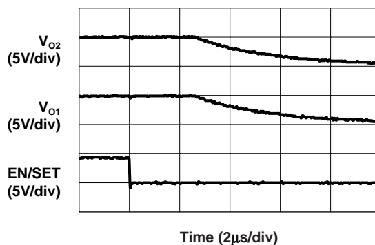
Turn-Off Characteristic ( V_{IN} = 5V ; R_{L1} = R_{L2} = 50\Omega ; C_{O1} = C_{O2} = 0.1\mu F )
