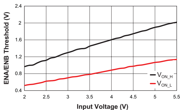
ENA/ENB Threshold vs. Input Voltage ( T_A = 25^\circ\text{C} )
