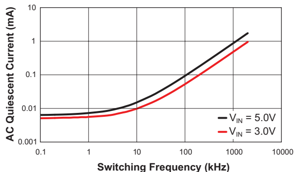
AC Quiescent Current vs. Switching Frequency (ENB = IN; ENA = 0.1kHz~2000kHz; I OUT = 0; T A = 25°C)
