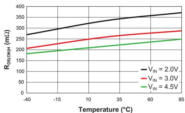
High Side R_{DS(ON)} vs. Temperature ( I_{OUT} = 0.7A )
