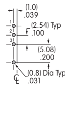
AB11 model does not have terminal 2. AB11AV1-FA
