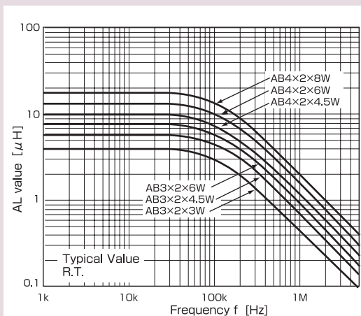
Frequency Characteristics of Inductance
