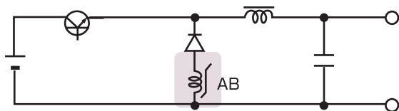
Chopper Converter
