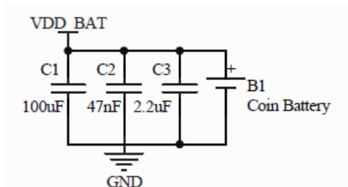
Figure 2. Capacitor at pin VDD_BAT
