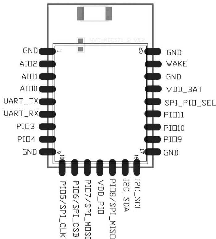
Figure 1. Pinout (Topview)
