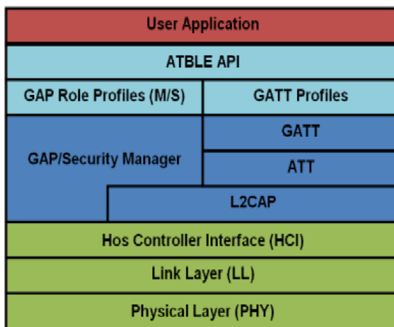
Figure 3. iNovaLE Stack
