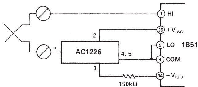
Figure 3. Using the AC1226 with the IB51, Isolated mV/Thermocouple Signal Conditioner
