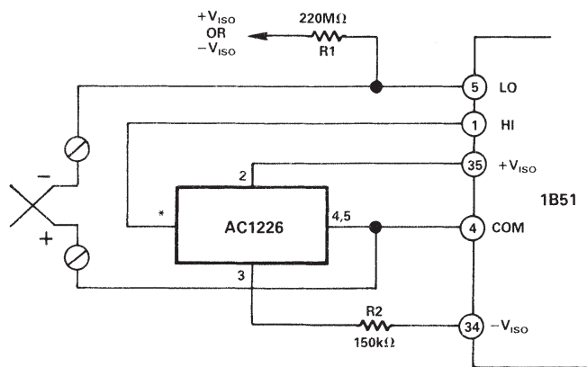
Figure 3. Using the AC1226 with the IB51, Isolated mV/Thermocouple Signal Conditioner
