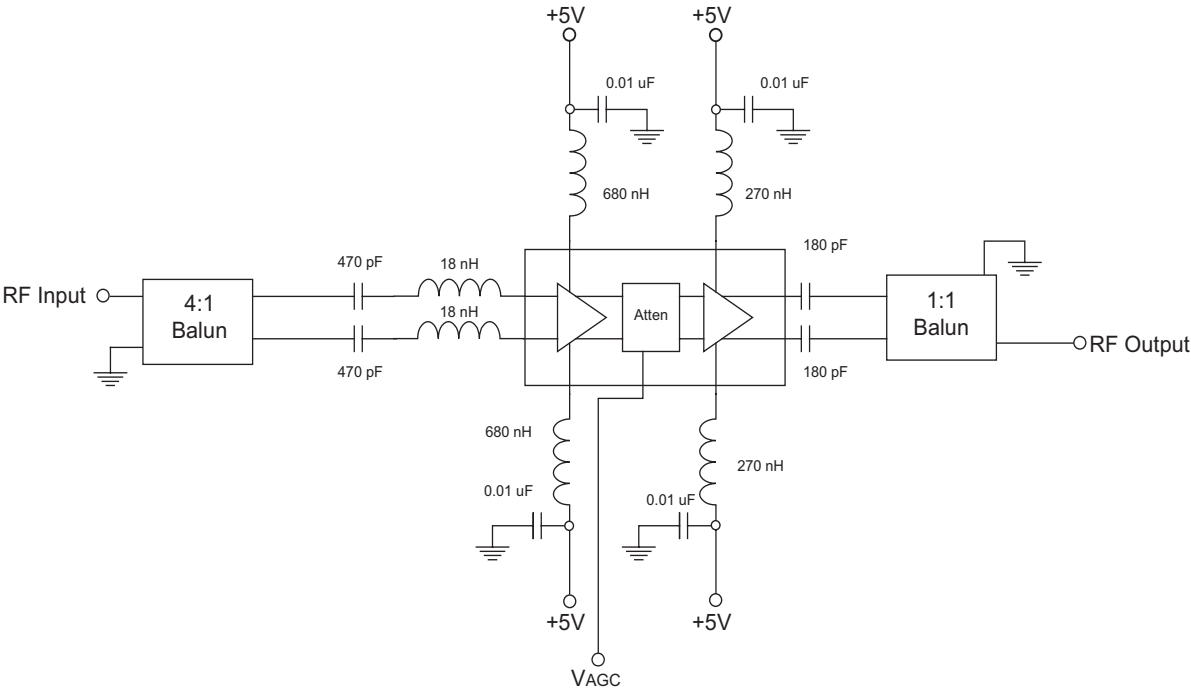
Figure 3: Test Circuit
