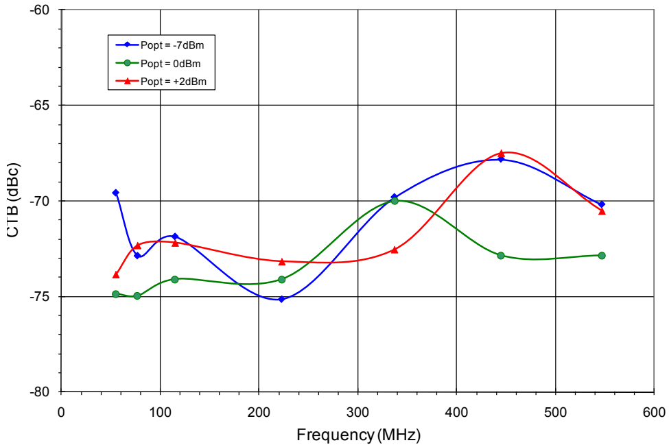
Figure 8: CTB vs. Frequency vs. P OPT (79 Analog channels (55.25 to 547.25 MHz), +17 dBmV at 109.25 MHz, 3.5% OMI/ch)
