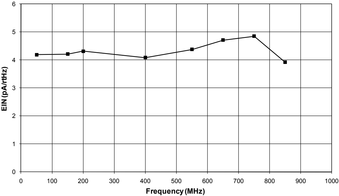
Figure 10: Equivalent Input Noise vs. Frequency (TA = 25 °C, VCC = +5 V, VAGC = +3.0 V)
