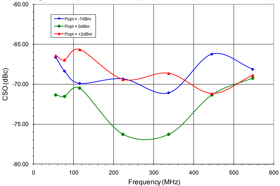
Figure 9: CSO vs. Frequency vs. P OPT (79 Analog channels (55.25 to 547.25 MHz), +17 dBmV at 109.25 MHz, 3.5% OMI/ch)
