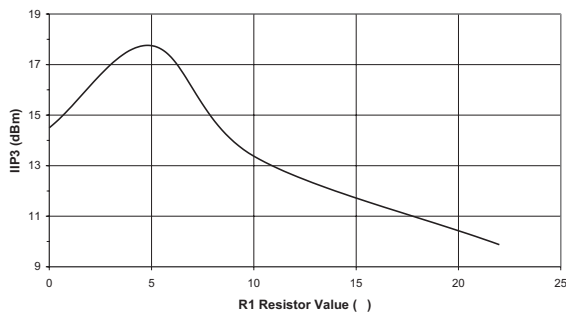
Figure 19: Typical Input IP3 vs. LNA/Mixer Current Control Resistor R1 ( T_A = +25^\circ\text{C} , V_{DD} = +5\text{ V} )
