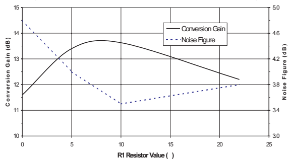
Figure 17: Typical Conversion Gain and Noise Figure vs. LNA/Mixer Current Control Resistor R1 ( T_A = +25^\circ\text{C} , V_{DD} = +5\text{ V} , f_{LO2} = 1042\text{ MHz} )
