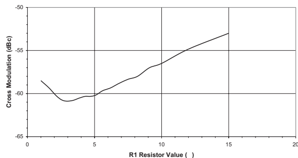
Figure 20: Typical Cross Modulation vs. LNA/Mixer Current Control Resistor R1 ( T_A = +25^\circ\text{C} , V_{DD} = +5\text{ V} )
