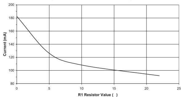
Figure 18: Typical Total Current Consumption vs. LNA/Mixer Current Control Resistor R1 ( T_A = +25^\circ\text{C} , V_{DD} = +5\text{ V} )
