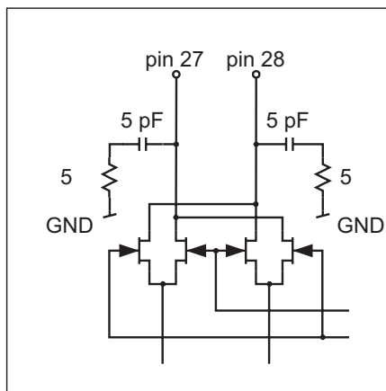
Figure 22: Equivalent Circuits
