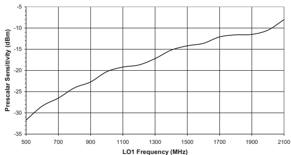
Figure 11: Typical Upconverter Prescaler Sensitivity vs. Local Oscillator Frequency ( T_A = +25^\circ\text{C} , V_{DD} = +5\text{ V} )
