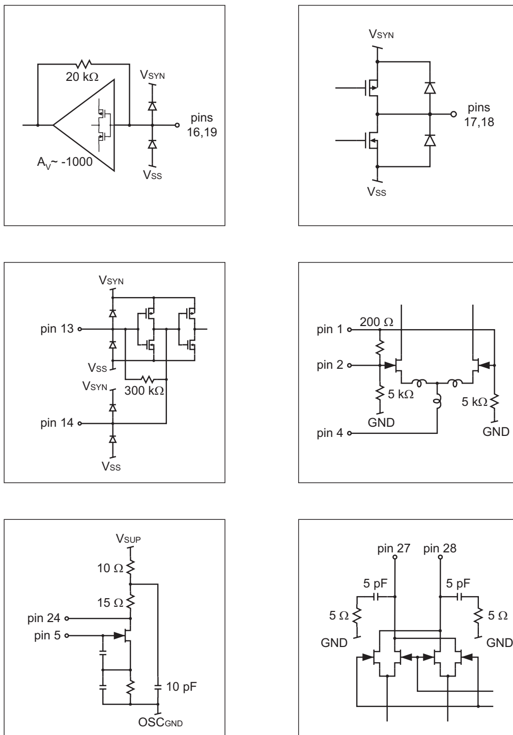
Figure 23: Equivalent Circuits
