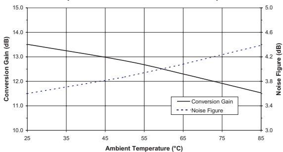
Figure 6: Typical Conversion Gain and Noise Figure vs. Ambient Temperature (V_{DD} = +5\text{ V}, f_{LO2} = 1042\text{ MHz})
