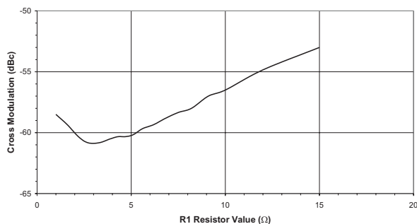
Figure 20: Typical Cross Modulation vs. LNA/Mixer Current Control Resistor R1 ( T_A = +25\text{ }^{\circ}\text{C} , V_{DD} = +5\text{ V} )
