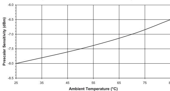
Figure 15: Typical Upconverter Prescaler Sensitivity vs. Ambient Temperature ( V_{DD} = +5\text{ V} , f_{LO1} = 2100\text{ MHz} )
