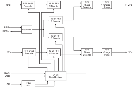
Figure 2: Dual Synthesizer Block Diagram
