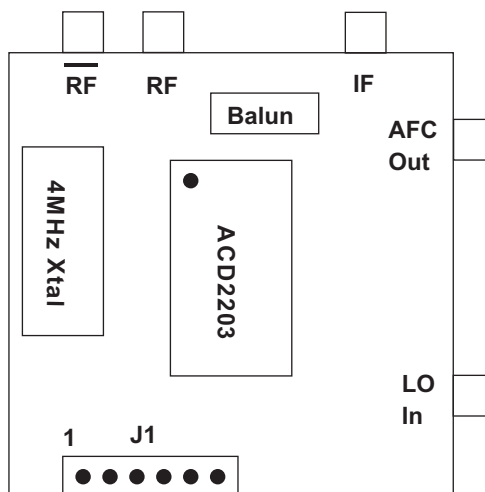
Figure 27: Evaluation Fixture
