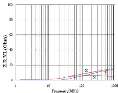
ACML-0805-070
