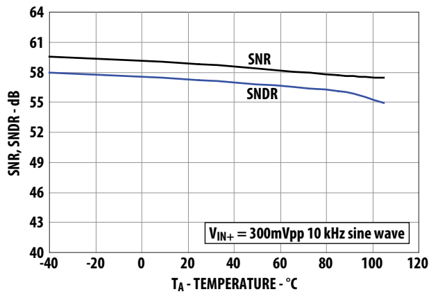
Figure 15. SNR, SNDR vs. temperature.
