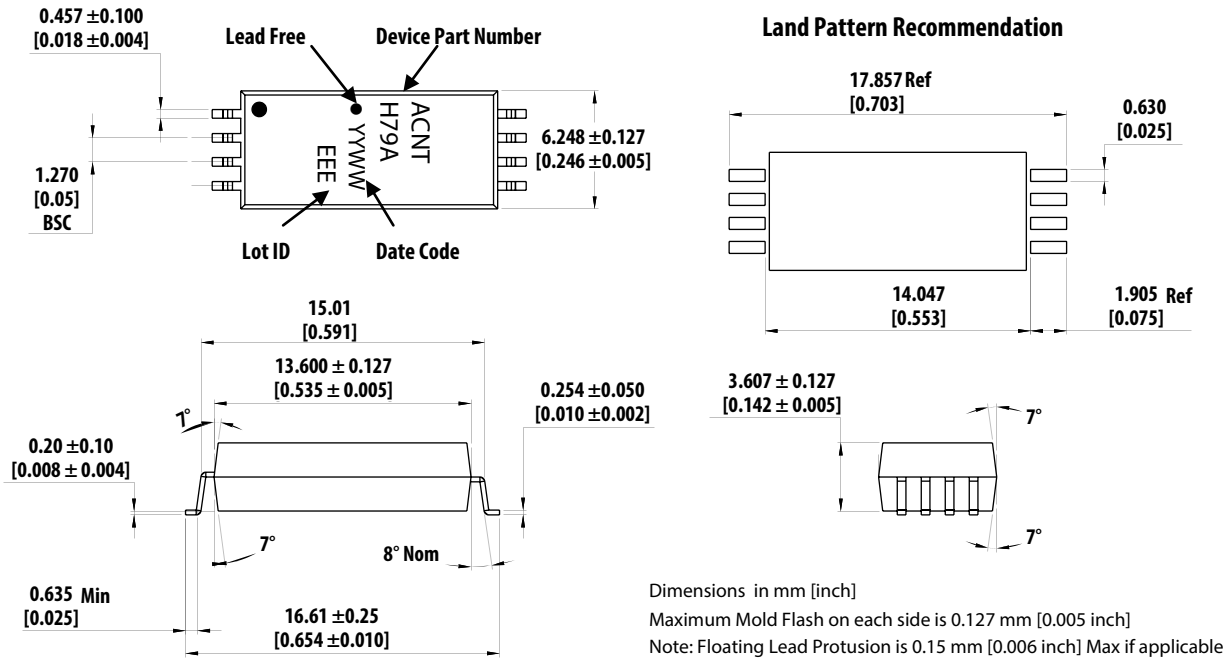
Figure 2. 14.2mm SO-8 Package
