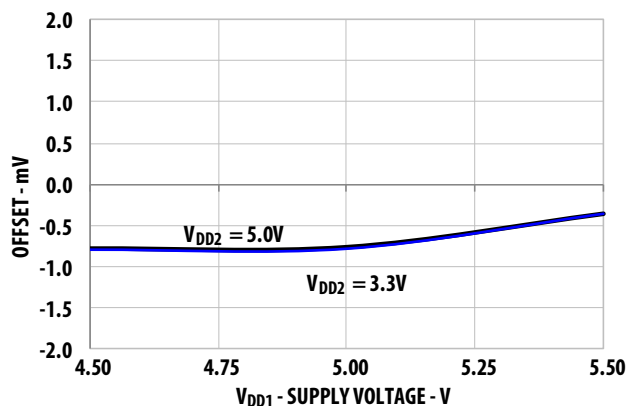
Figure 3. Input offset vs. supply V_{DD1}
