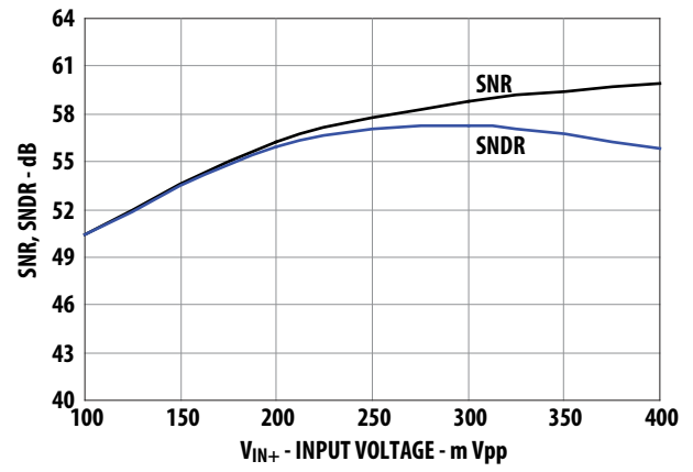
Figure 16. SNR, SNDR vs. input voltage.
