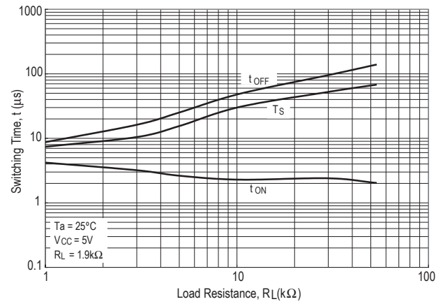
Figure 16. Switching Time vs. Load Resistance
