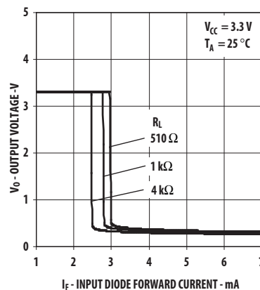
Figure 2. Input-Output Characteristics.
