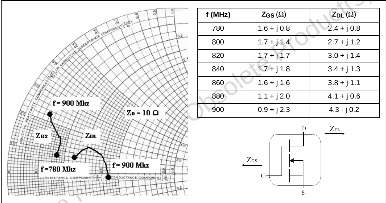
Figure 2. Impedance data
