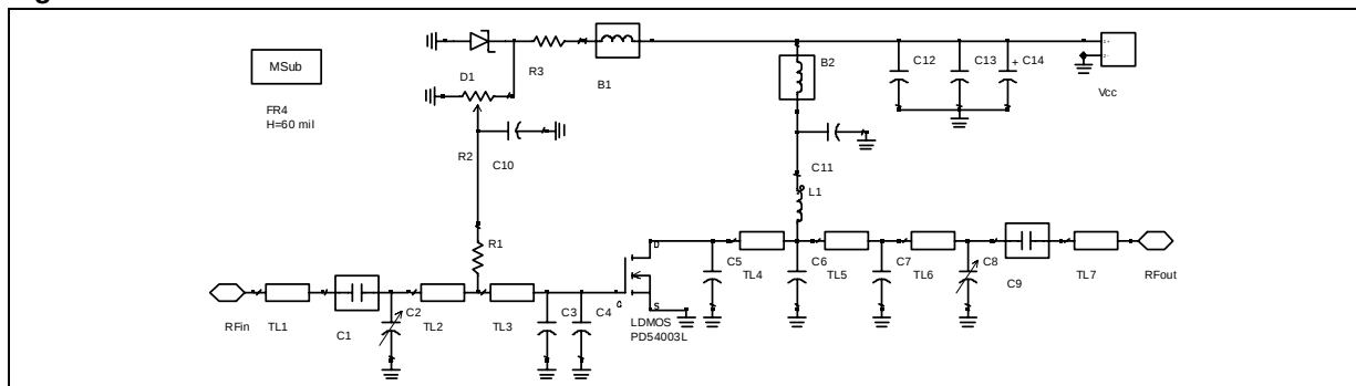
Figure 9. Test Circuit
