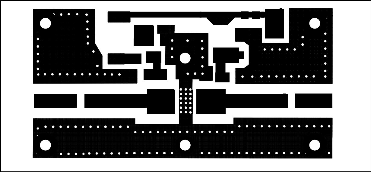
Figure 10. Photomaster
