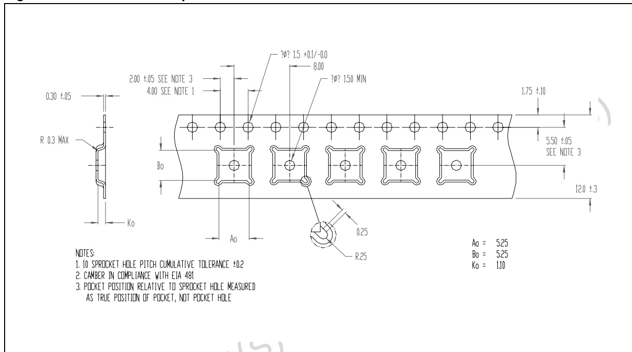
Figure 12. PowerFLAT™ Tape &amp; Reel
