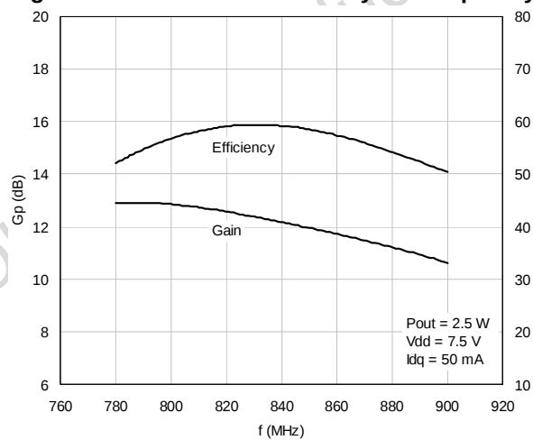
Figure 7. Pow. Gain &amp; Efficiency Vs Frequency
