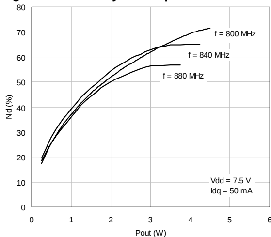
Figure 6. Efficiency Vs Output Power
