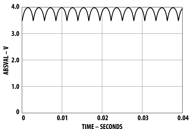
Figure 22. ABSVAL with 3 phases, wired-ORed together.
