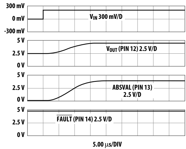
Figure 14. Step response, 0 to 200 mV input, at V_{REF} = 5 V.
