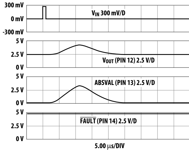
Figure 17. \overline{\text{FAULT}} rejecting a 1 \mu\text{s} , 0 to 2 V to 0 input. Rejection is independent of amplitude.
