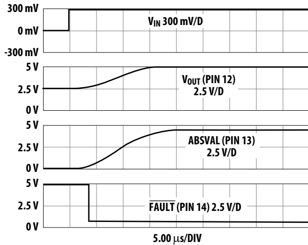
Figure 15. \overline{\text{FAULT}} detection, 0 to 300 mV input, at V_{\text{REF}} = 5 \text{ V} .
