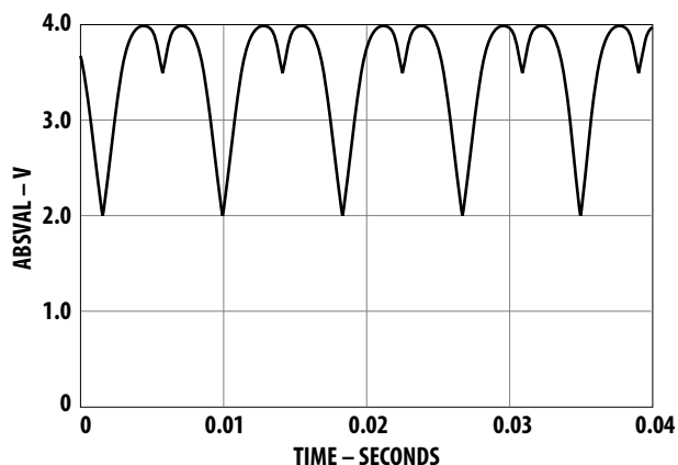
Figure 23. ABSVAL with 2 phases, wired-ORed together.
